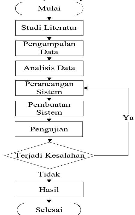
Gambar 4. Flowchart Penelitian
