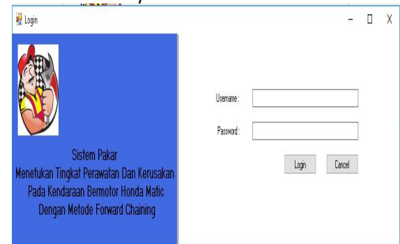
Form Login
