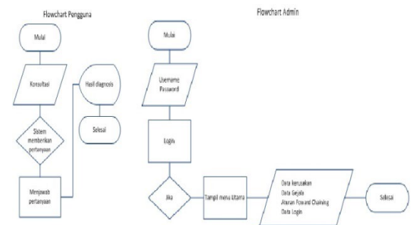
Flowchart sistem
